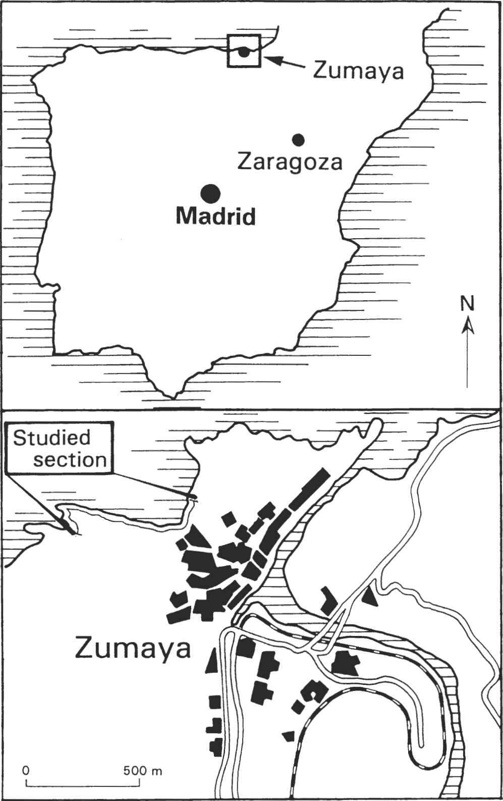
Fig. 1. Location of studied section.
