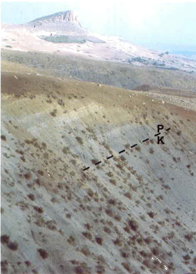
Plate 3 — The Ain Settara section, looking north, with in the background the nummulitic limestone cliffs of Sidi Nasseur.
