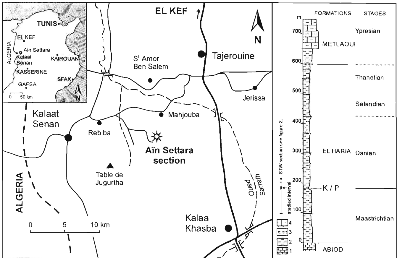
Fig. 1 — Location maps and general stratigraphical context of the studied intervals. The Abiod Formation is composed of limestones (1). The El Haria Formation is dominantly marly, sometimes clayey, with few calcareous beds (2). The Metlaoui Formation is dominantly calcareous (4); its base contains several phosphatic beds (3).
