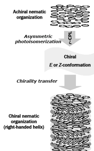
Fig.1 Proposed model for the photoinduction of chirality in azomaterials.
